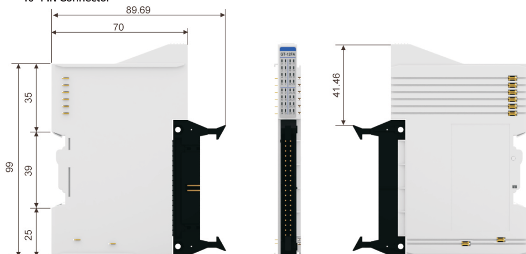
40-PIN Connector
