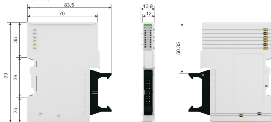
20-PIN Connector
